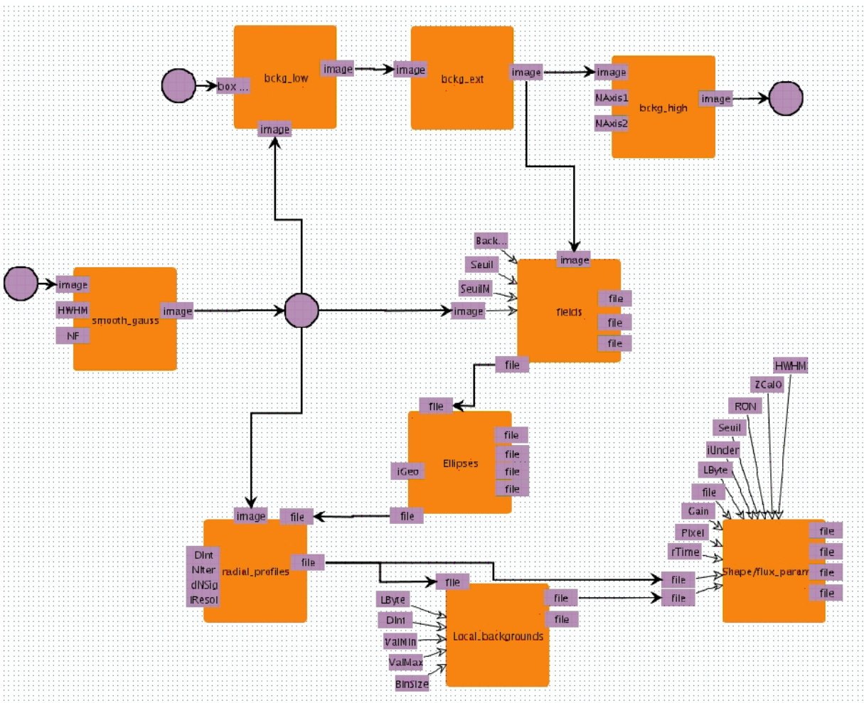
Fig. 1. A solution with AIDA.
