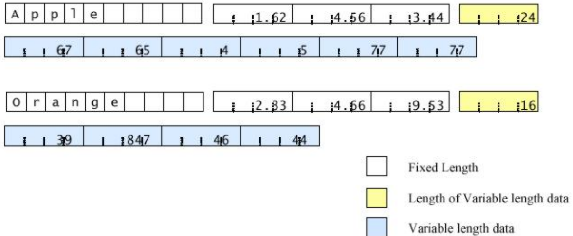
Figure 2: Data Storage in BINARY mode
